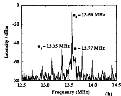
FIG. 4. The frequency spectrum obtained at E.P. showing (a) the low-frequency wave and (b) the upper and lower sideband peaks which are displaced from the rf pump frequency (13.56 MHz) by its frequency. Experimental conditions are 3 mTorr and 400 W.
