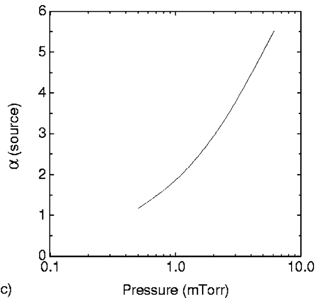
FIG. 6. Electron density (a), electron temperature (b), and electronegativity (c) in the center of the source and as a function of pressure, and for the same conditions as in Fig. 5. The symbols stand for the experiments while the lines are for the model.
